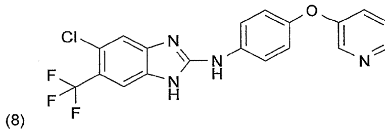
(5-Chlor-6-trifluormethyl-1H-benzimidazol-2-yl)-[4-(pyridin-3-yloxy)-phenyl]-amin
